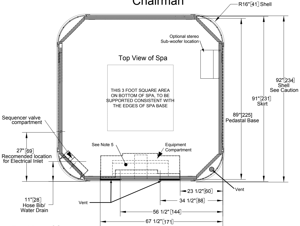
Top View of Spa
